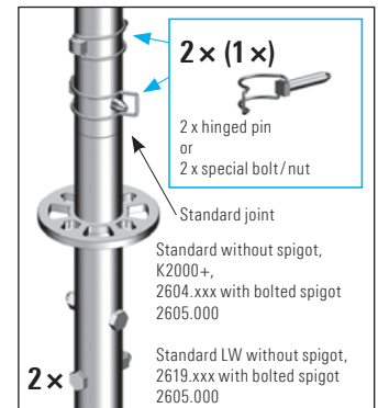
Fig. 88b: Tensile joint with bolted spigot
