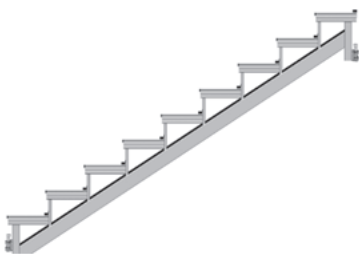
U-stairway stringer 500, 9 steps, Ref. No. 2638.009, 2.00 x 2.57 m
